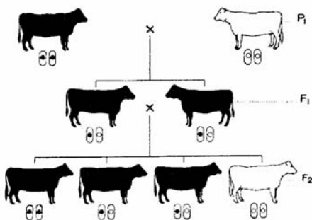
Black × Red. (Red is necessarily white in the diagram.)
