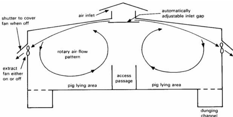
The NIAE ventilation system.
